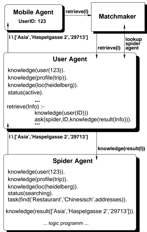
Figure 4: Agent Communication
