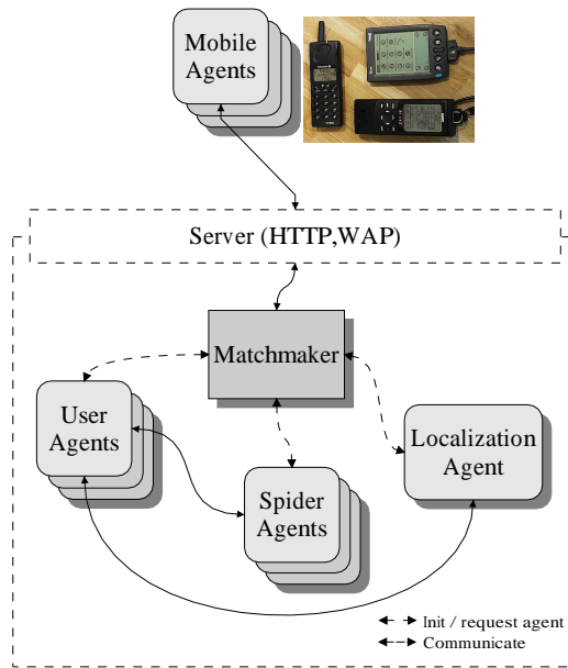
Figure 1: system architecture
